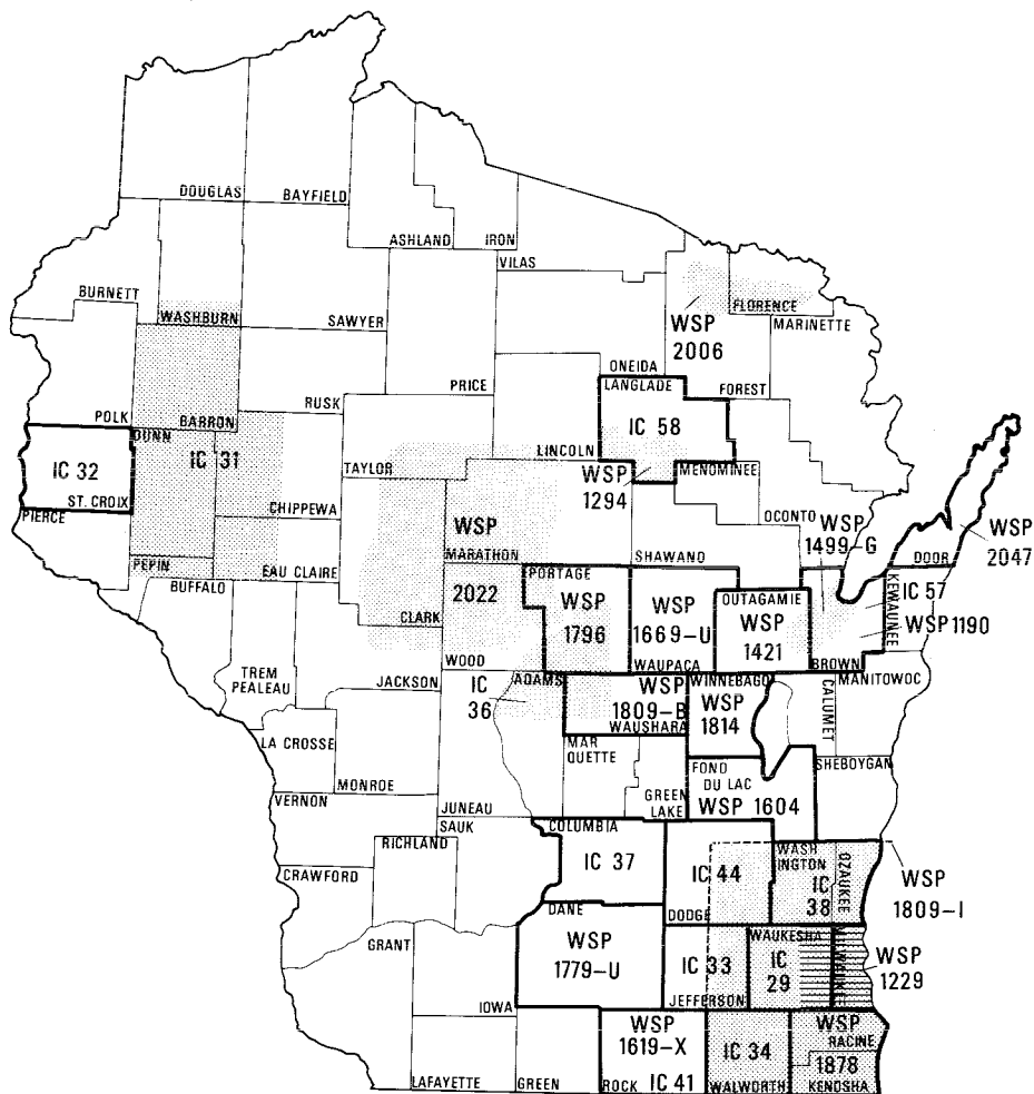
Figure 5. Published regional and county hydrogeologic studies (WSP = Water-Supply Paper, published by the U.S. Geological Survey; IC = Information Circular, published by the Wisconsin Geological and Natural History Survey).
