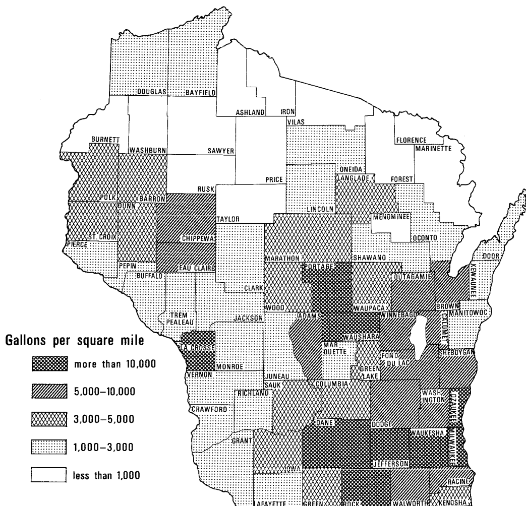
Figure A4. Groundwater use in Wisconsin in 1979, by county, in gallons per square mile (data source, Lawrence and Ellefson, 1982).
